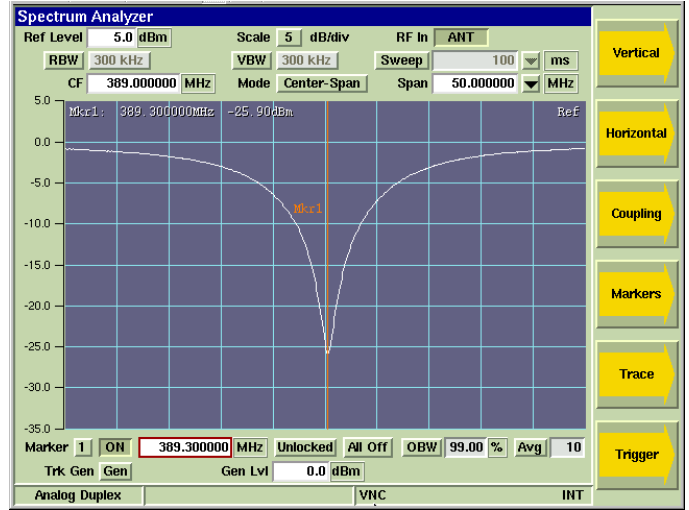
Figure 8. Spectrum Analyzer with Tracking Generator
