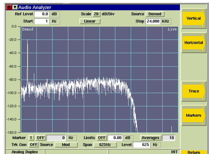
Figure 6. Audio Analyzer
