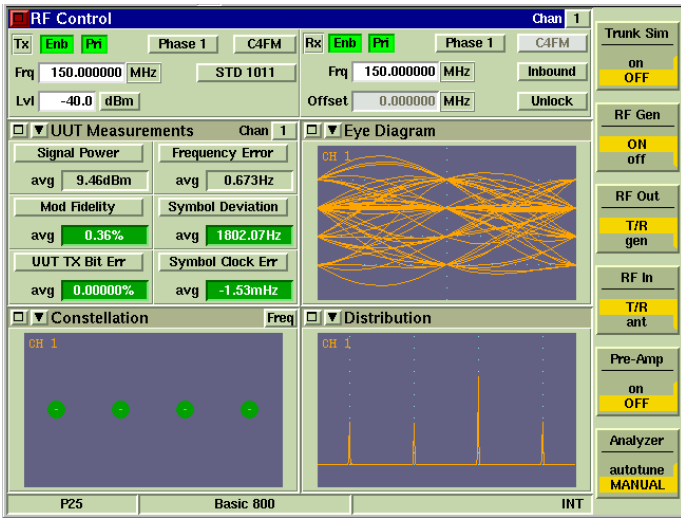
Figure 10. P25 Conventional
